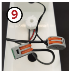
9 USE 2 PORT CONNECTORS TO CONNECT THE WIRES FROM THE POWER SUPPLY (RED TO RED + BLACK TO BLACK) YOU'RE NOW READY TO CONNECT THE BROWN + BLUE TO THE MAINS
