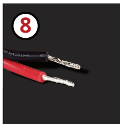
8 AT THE END LEAVE 100MM OF CABLE - STRIP 10MM OF RED + BLACK TO BARE WIRE
