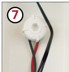
7 SCREW THE LAMP HOLDER NUT DOWN ON THE CABLES TIGHTLY TO MAKE THE CONNECTION
